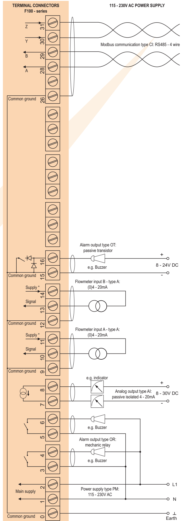
Typical wiring diagram F114-A-AI-CI-OR-PM
